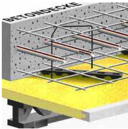
Figure 3 - cross-section of a TMA on-site constructed system (www.velta.de).
