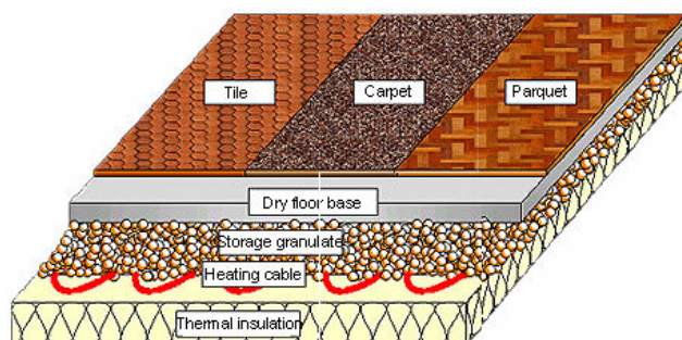
figure 5 – Example of an under floor heating and cooling system with PCM (Rubitherm).
