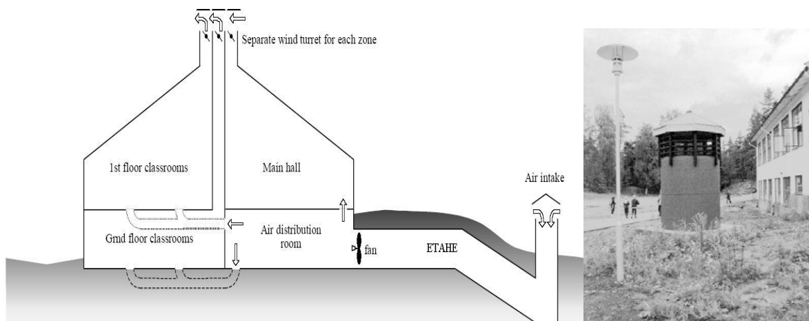
Figure 4 - Example of an EC system - schematic cross section of Jaer School (NO).
