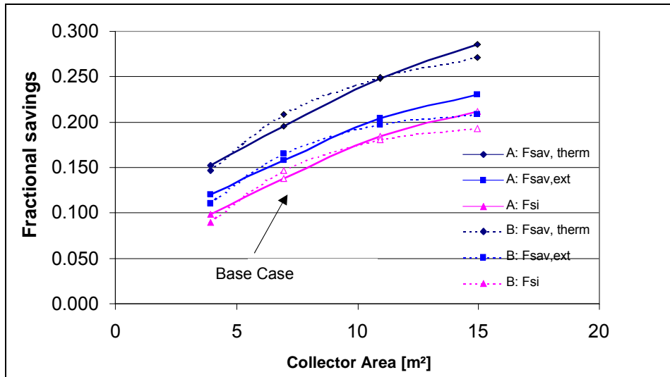
Figure 20 Dependency of f_{sav} on collector area with fixed store volume ( 0.28 \text{ m}^3 ), example of system #2. Control strategy A: boiler running all year, B: electric immersion heater used in summer [6]
