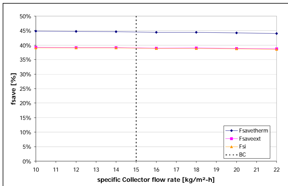
Figure 21 Dependency of f_{sav} with specific collector flow rate, example of system #19 (stratification unit in storage) [14]
