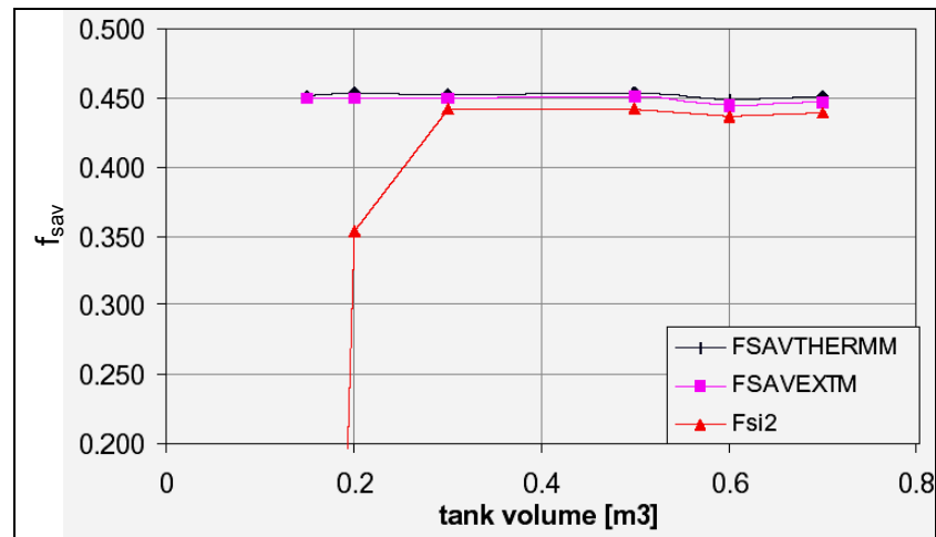
Figure 24 Dependency of f_{sav} with DHW store volume, system #3a (20 m 2 collector area, 0.5 m 3 DHW store and floor heating system with 10 cm thickness) [7]
