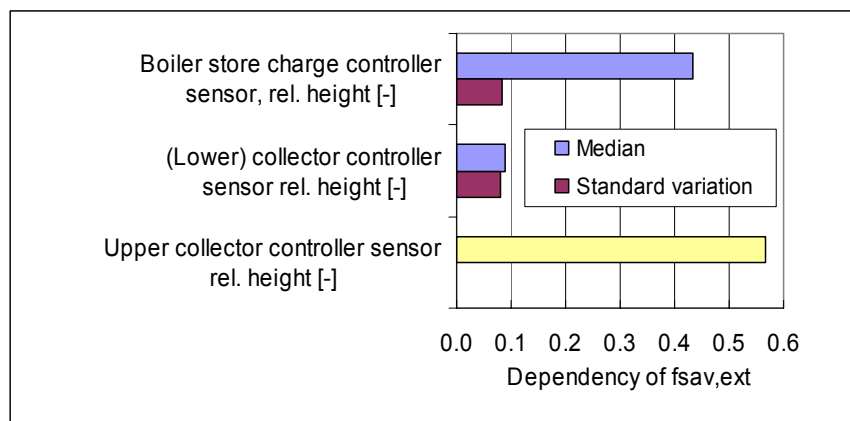
Figure 50 Dependency of f_{sav,ext} on specific parameter change of temperature sensor positions
