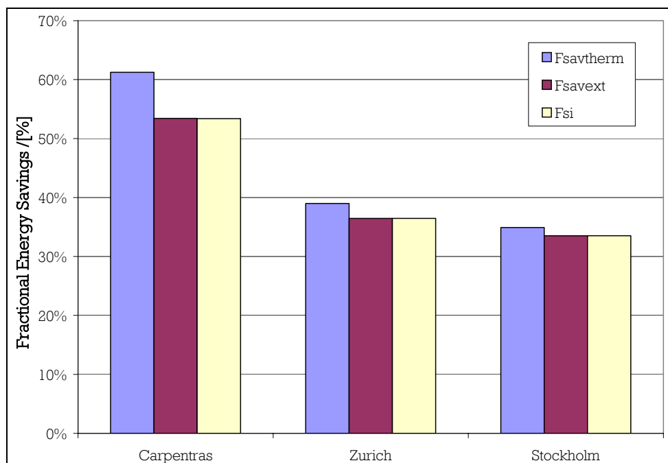
Figure 15 f_{sav} for different climates and SFH60 building, system #15, 10 m 2 collector area, 0.635 m 3 store volume [13]
