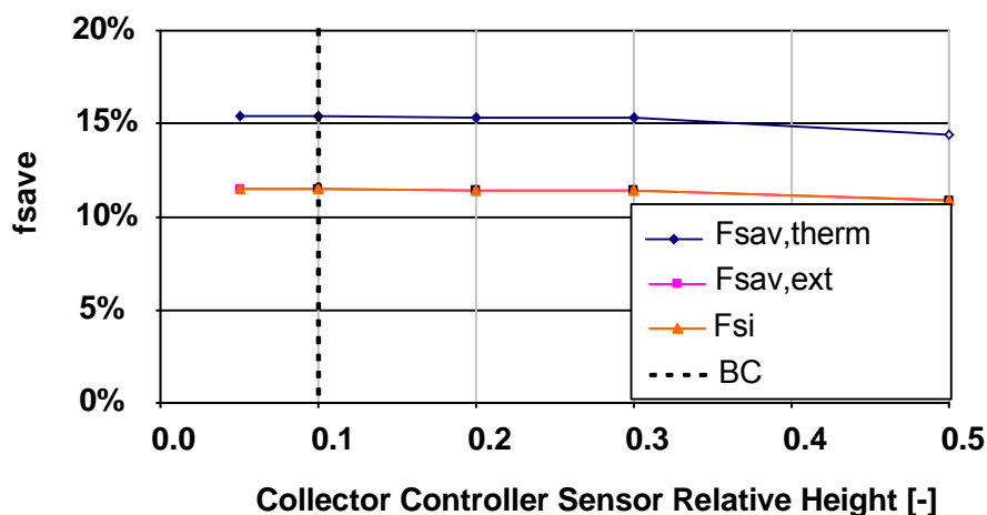
Figure 37 Variation of f_{sav} with variation of collector controller's temperature sensor position example of system #11, (0.036 = collector outlet, 0.2 collector inlet) [11]
