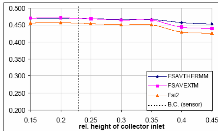
Figure 34 Variation of f_{sav} with variation of solar collector heat inlet height, example of system #3a, spec. collector mass flow 40 \text{ kg}/(\text{m}^2_{\text{collector},h}) [7]
