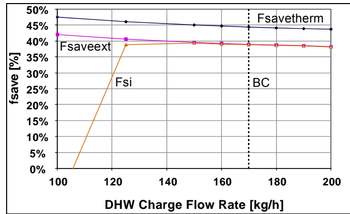
Figure 40 Variation of f_{sav} with variation of specific mass flow rate from SH store to DHW store, system #19, [14]
