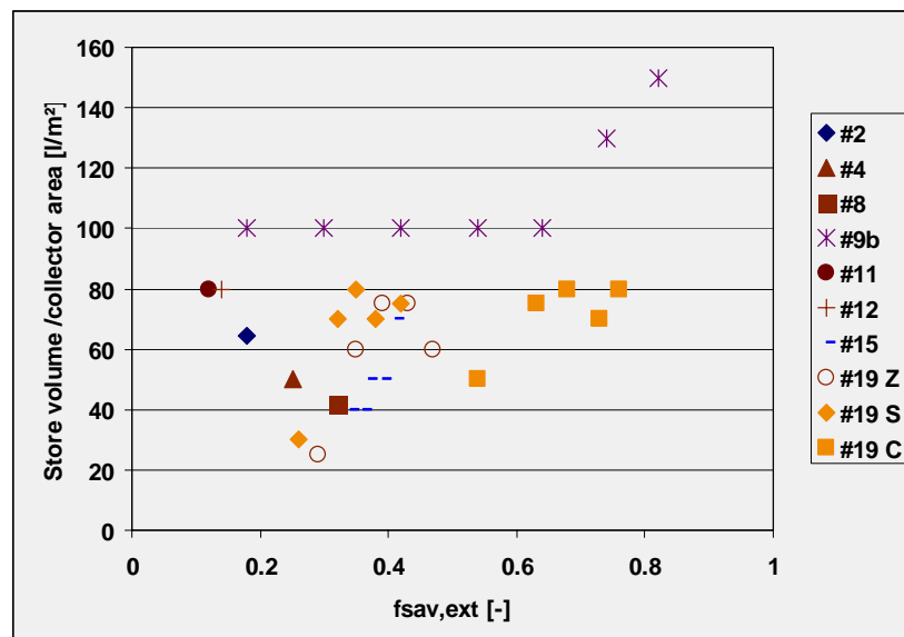
Figure 27 Optimal ratio of store volume and collector size for different f_{sav,ext} for all systems analyzed.
