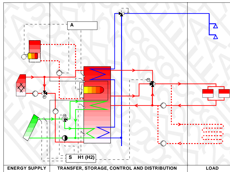
Figure 8 System #12, hydraulic design
