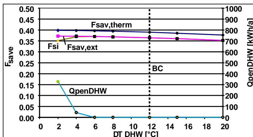
Figure 42 Variation of f_{sav} with variation of DHW set point temperature for auxiliary boiler, relative to DHW draw off temperature, system #15, [13]
