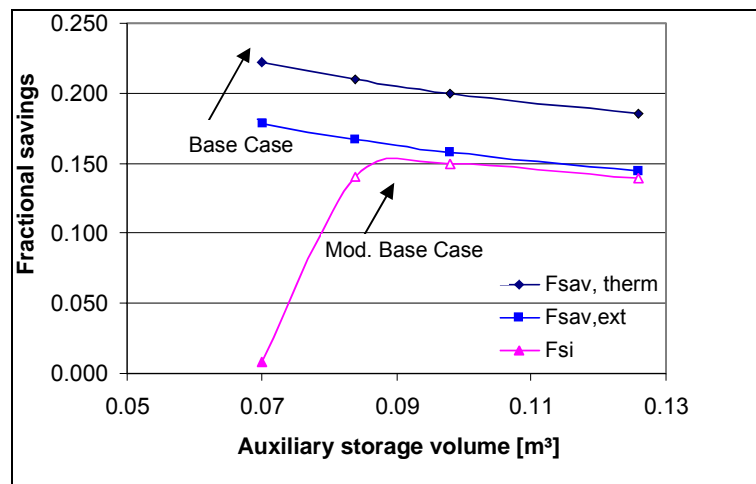
Figure 32 Variation of f_{sav} with variation of auxiliary heater volume example of system #2, internal heat exchanger [6]
