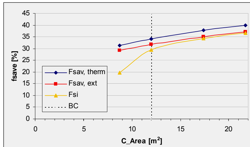
Figure 26 Variation of f_{sav} with collector size with fixed specific store volume of 0.069 m 3 /m 2 , example of system #4 [8].
