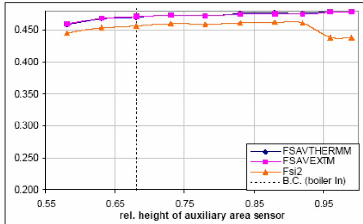
Figure 38 Variation of f_{sav} with variation of relative height of auxiliary boiler sensor, example of system #3a, pure DHW store [7]
