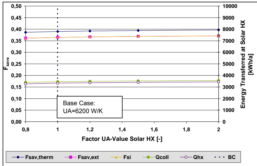
Figure 29 Dependency of f_{sav} with collector heat exchanger UA value, example of system #15 [13]
