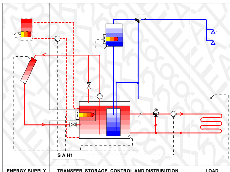
Figure 5 System #9b, hydraulic design
