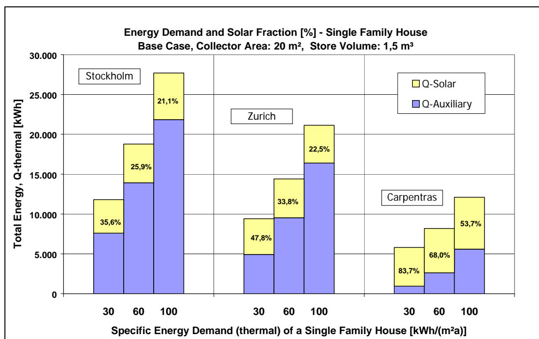
Figure 16 Total energy ( Q_{\text{thermal}} ) and f_{\text{sav,therm}} for different insulation standards and locations. System #9b: Base Case [10]
