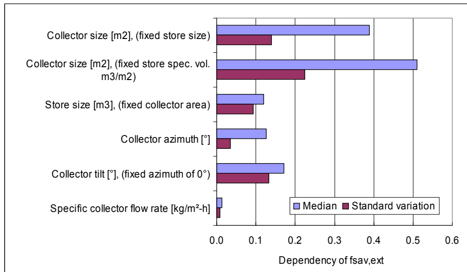
Figure 46 Dependency of f_{sav,ext} on specific parameter change of collector and store size
