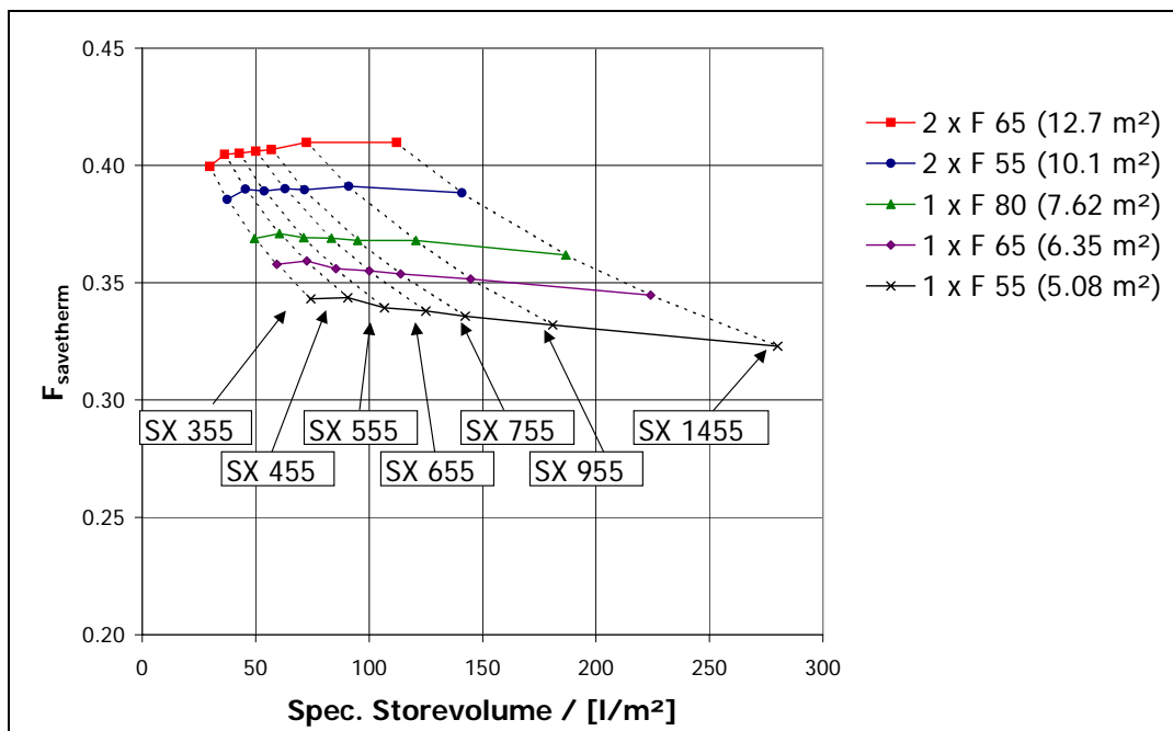
Figure 25 Dependency of f_{sav,therm} with store volume and collector area, example of system #15 [13]
