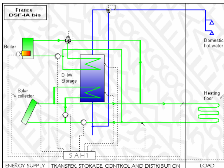
Figure 2 System #3a, hydraulic design
