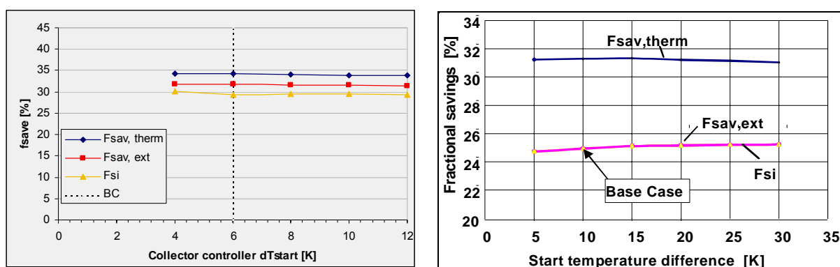
Figure 22 Dependency of f_{sav} with the collector controller settings, example of system #8 [9] (left) for a SH store and system #4 [8] (right) for a DHW store.
