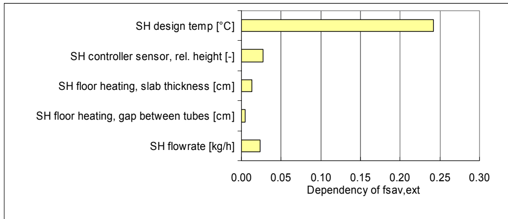
Figure 51 Dependency of f_{sav,ext} on specific parameter change of temperature sensor positions, system #3 [7]
