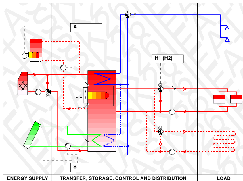
Figure 7 System #11, hydraulic design
