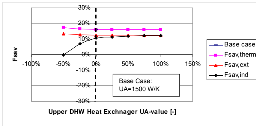
Figure 30 Dependency of f_{sav} with upper internal DHW heat exchanger UA value, example of system #12 [12]
