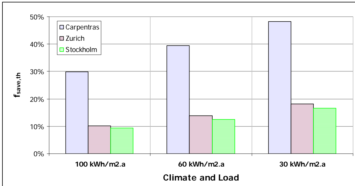
Figure 14 Dependency of f_{sav,therm} on climate and building, system #11, 10 m 2 collector area, 0.73 m 3 store volume [11].
