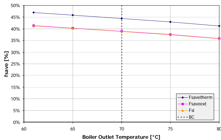
Figure 44 Variation of f_{sav} with the internal standby temperature of the oil boiler. This is also the set outlet temperature of the boiler, system #19, [14]
