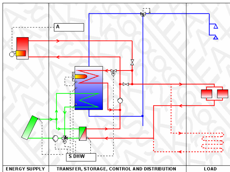
Figure 1 System #2, hydraulic design
