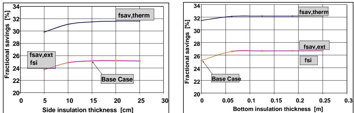
Figure 28 Variation of f_{\text{sav}} with thickness of side and bottom insulation of storage tank, example of system #4 [8].
