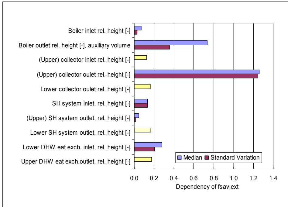
Figure 47 Dependency of f_{sav,ext} on specific parameter change of storage geometry
