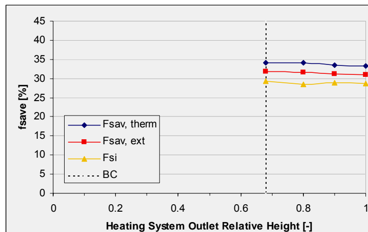
Figure 36 Variation of f_{sav} with variation of SH outlet height, example of system #8, gas burner mounted [9]
