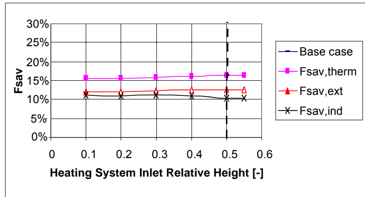
Figure 35 Variation of f_{sav} with variation of SH inlet height, example of system #12, flow inlets and outlets [12]
