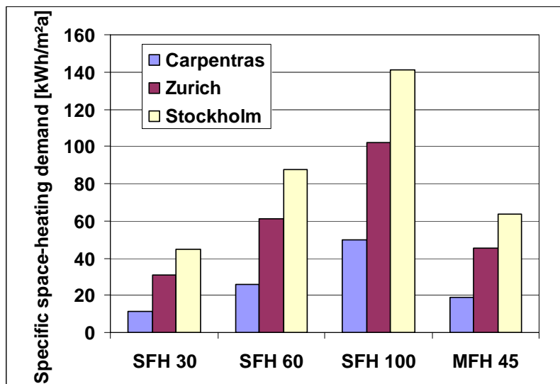
Figure 12 Specific space heating demand for the reference buildings [1].
