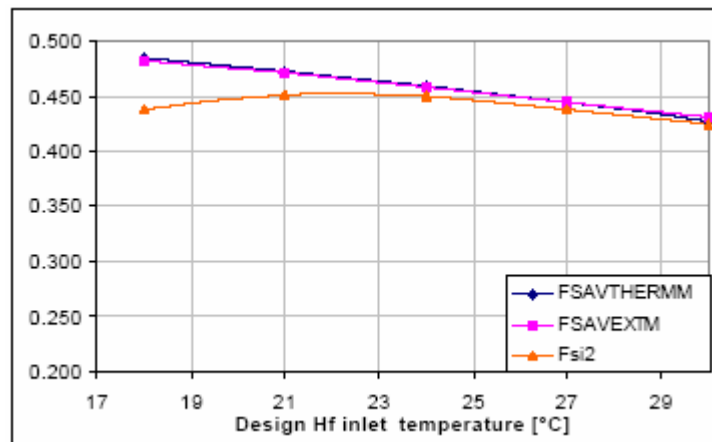
Figure 45 Variation of f_{sav} with variation of design heating floor inlet temperature, system #3a [7].
