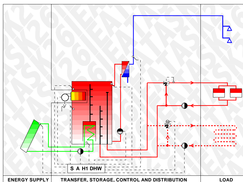
Figure 9 System #15, hydraulic design
