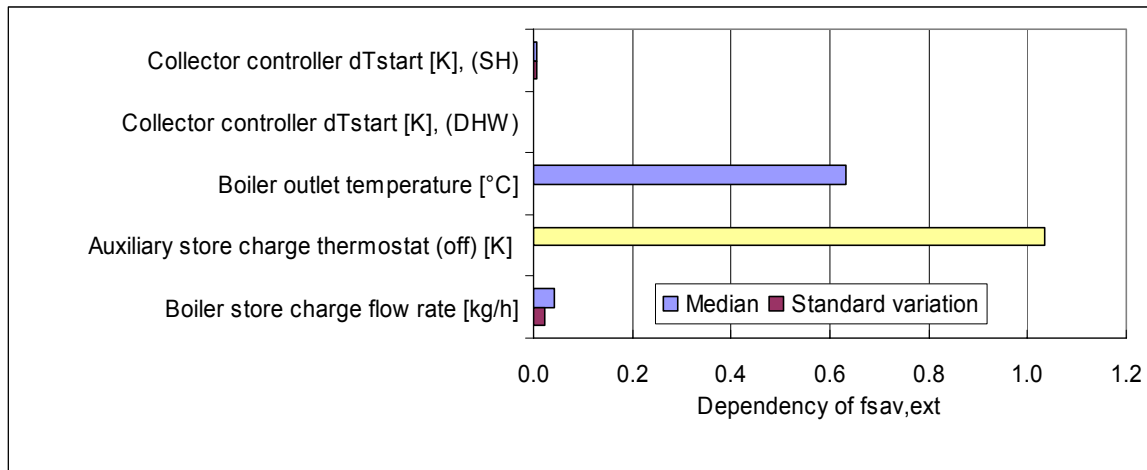
Figure 49 Dependency of f_{sav,ext} on specific parameter change of control settings and auxiliary boiler data
