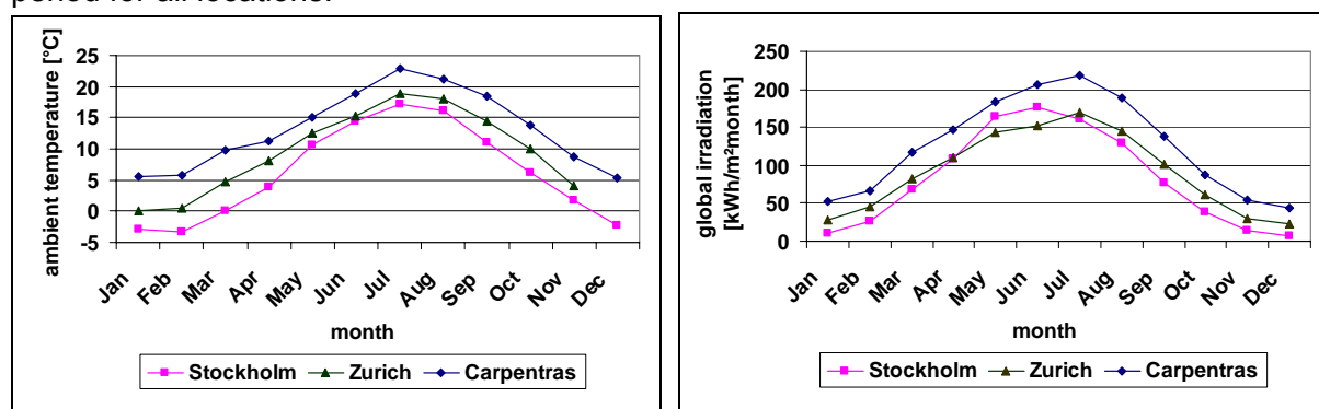
Figure 11 Monthly global irradiation (on a horizontal surface) and ambient temperature of the climates chosen in Task 26 [1]
