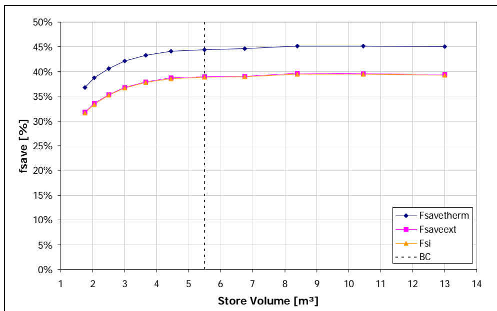
Figure 23 Dependency of f_{sav} with store volume, example of system #19 [14]
