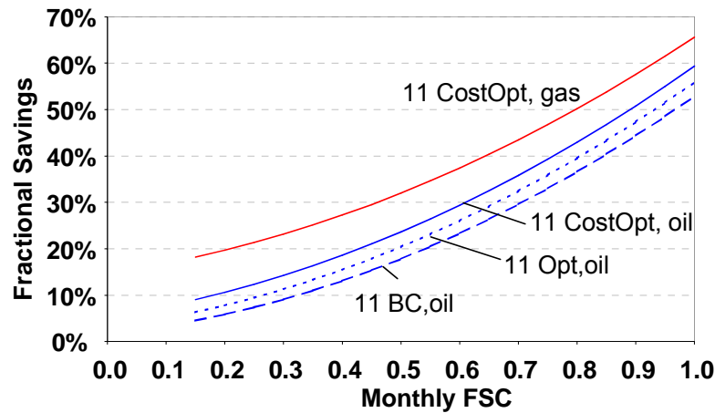
Figure 43 FSC characteristics for system 11 based on 3 climates (Carpentras, Zurich, Stockholm), 3 loads (30, 60, 100 kWh/m 2 a single family buildings and three collector sizes (5, 10, 20 m 2 ), system #11 [11].
