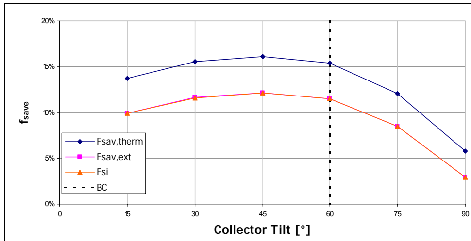
Figure 18 Dependency of f_{sav} on collector tilt, with fixed azimuth angle of 0^\circ , system 11, [11]
