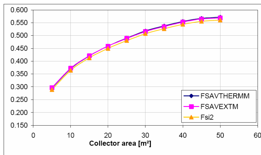
Figure 19 Dependency of f_{sav} on collector area with fixed store volume, example of system #3a ( 0.5 m^3 DHW store and floor heating system with 10 cm thickness) [7]
