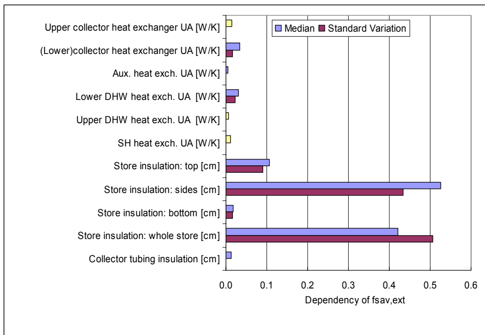
Figure 48 Dependency of f_{sav,ext} on specific parameter change of heat exchangers and store insulation
