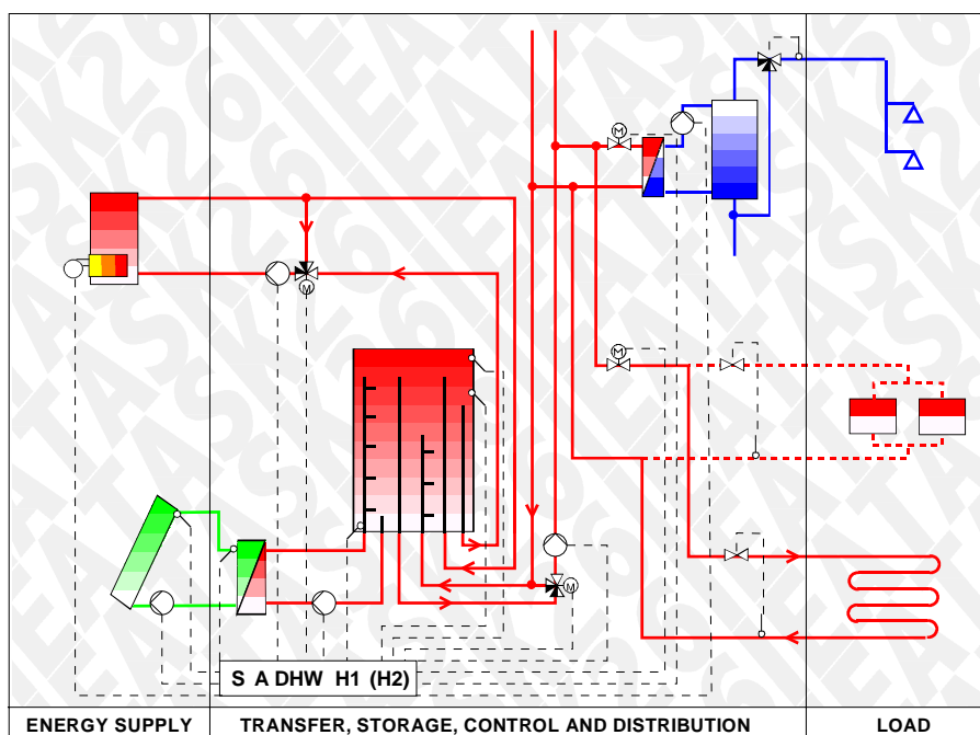
Figure 10 System #19, hydraulic design
