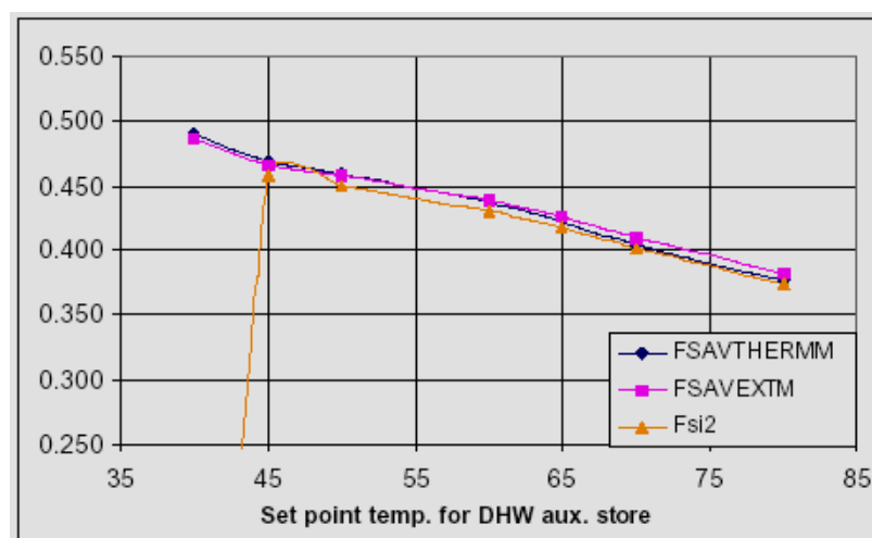
Figure 41 Variation of f_{sav} with variation of DHW set point temperature for auxiliary boiler, system #3a, [7]
