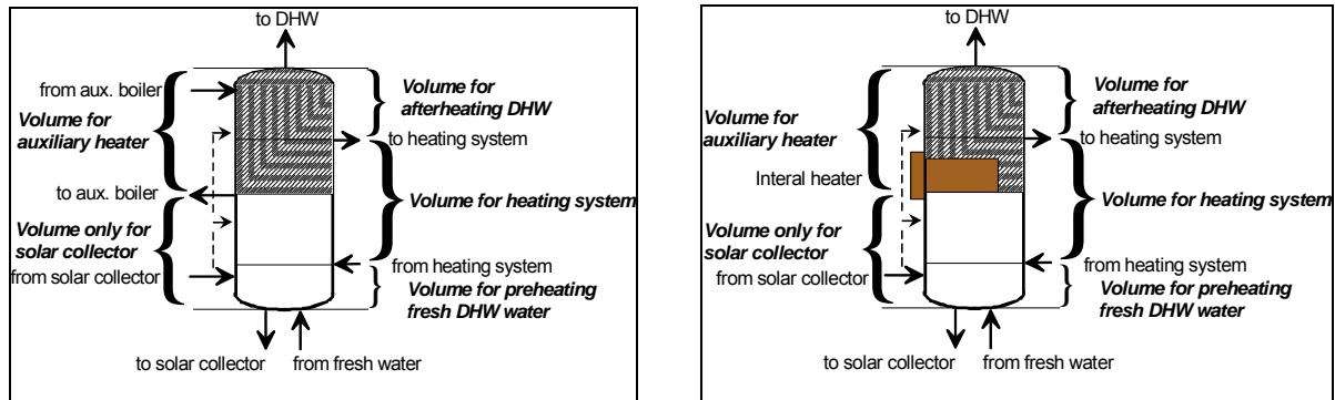
Figure 31 Different volumes in a combistore for auxiliary heat for external (left) and internal (right) heater
