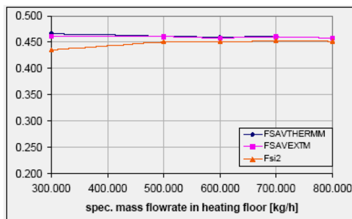
Figure 39 Variation of f_{sav} with variation of specific mass flow rate of the SH system, system #3a, [7]
