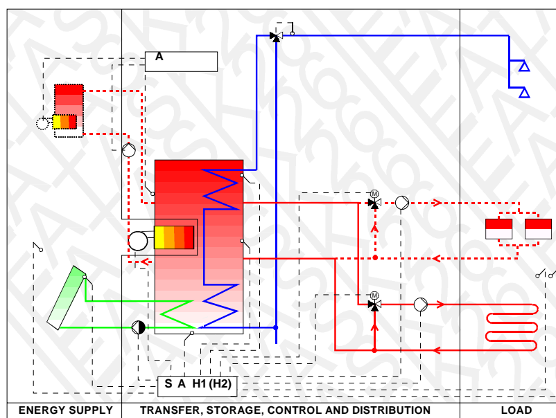
Figure 4 System #8, hydraulic design
