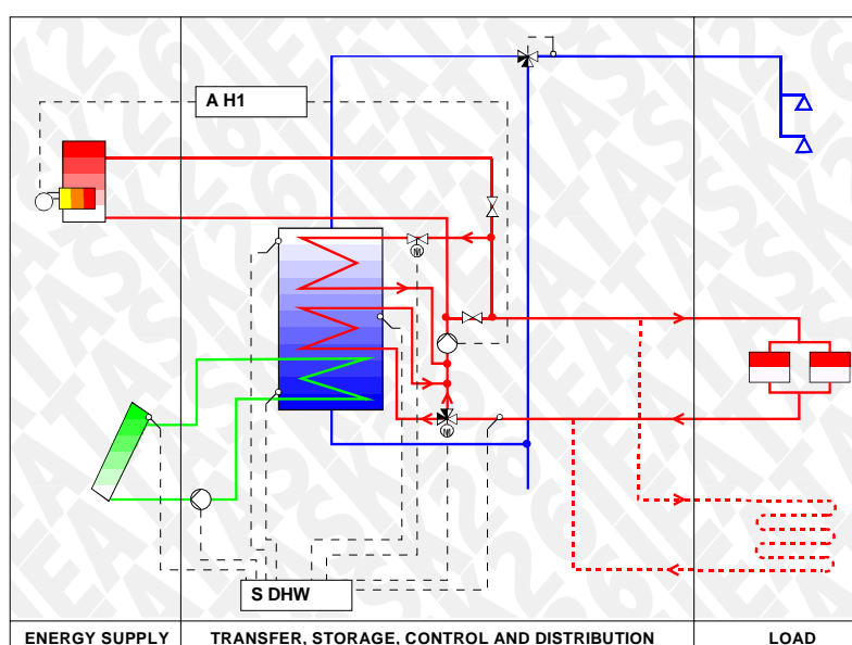
Figure 3 System #4, hydraulic design
