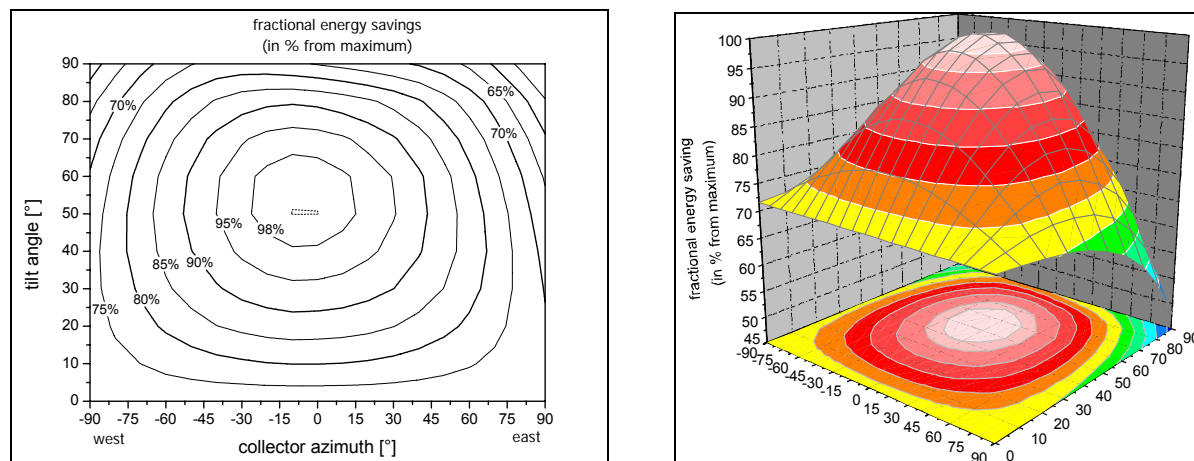
Figure 17 Dependency of f_{sav,ext} on collector tilt and azimuth angle. 100% \cong 39.4% ( f_{sav,ext} ), system #19 [14]
