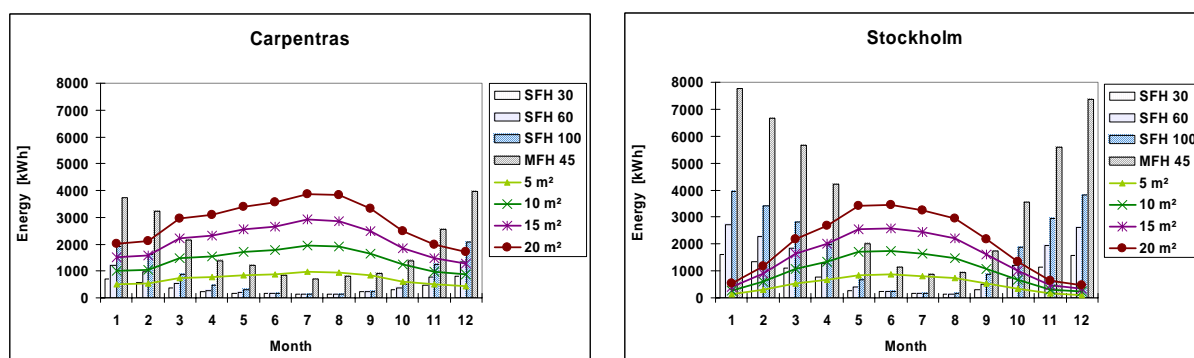
Figure 13 Monthly space heating and domestic hot water demand for the reference buildings and incident solar energy on different collector areas (facing south, slope of 45°) for Carpentras and Stockholm climates.
